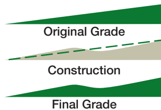
Broad-based Dip Cross-section
